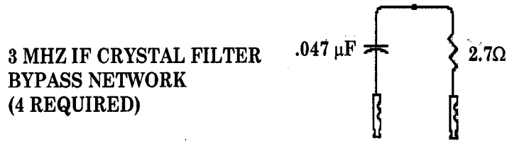
Figure 10. Filter.
