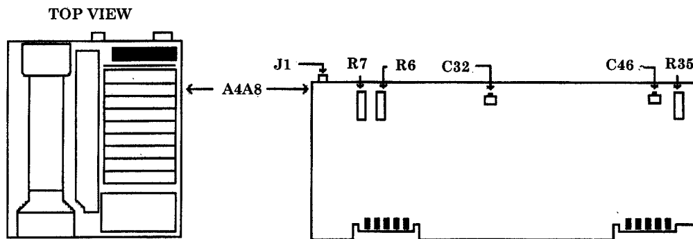
Figure 13. A4A8 board.
