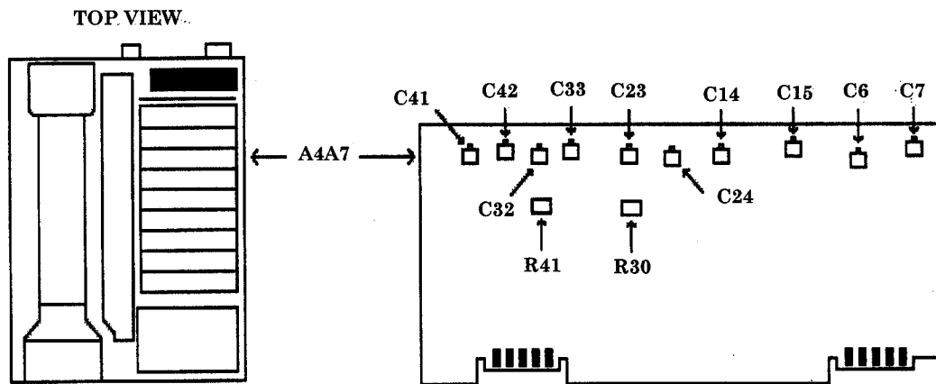
Figure 12. A4A7 board.
